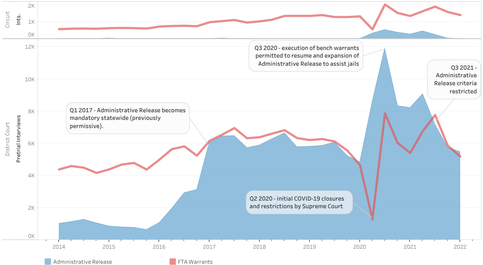
Comparison of Administrative Release and Failure to Appear Warrants AR: Pretrial Interviews with Release Outcome Administrative Release with Custody Ending 1/1/2014 - 3/31/2022 Statewide FTA Warrants: Pretrial Interviews (all Release Outcomes) with FTA Outcome Warrant Info and FTA Date 1/1/2014 - 3/31/2022 Statewide
